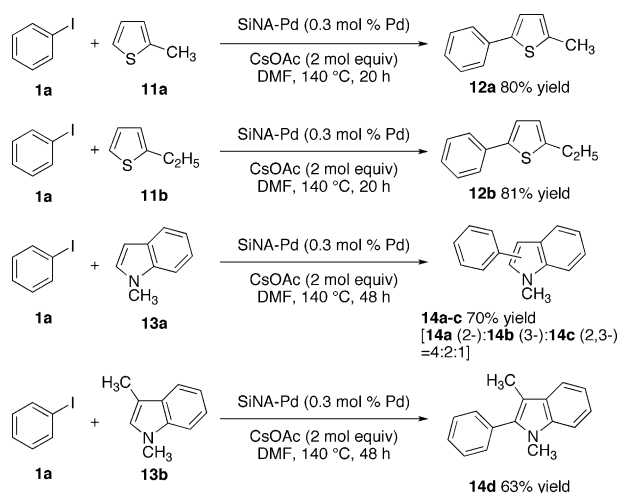
Scheme 3. C–H bond functionalization reactions of thiophenes and indoles.
