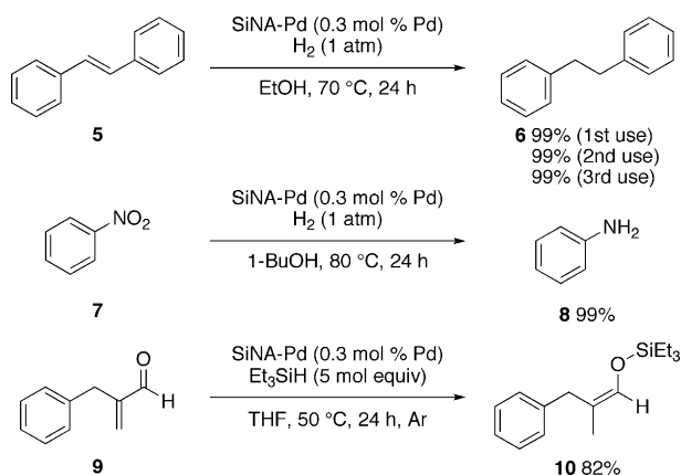
Scheme 2. Hydrogenation of stilbene, hydrogenolysis of nitrobenzene, and hydrosilylation of an \alpha,\beta -unsaturated aldehyde.
