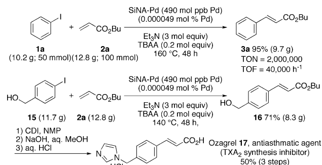
Scheme 4. Mizoroki–Heck reaction with 490 mol ppb (0.000049 mol %) Pd of SiNA-Pd, and the synthesis of Ozagrel, an antiasthmatic agent.
