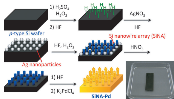
Scheme 1. Preparation of the SiNA-stabilized Pd nanoparticle catalyst (SiNA-Pd).
